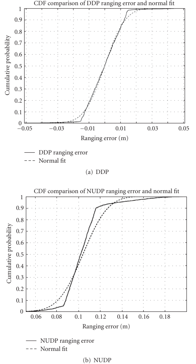
FIGURE 5: Distribution modeling of the ranging error with normal distribution for (a) DDP class of receiver locations and (b) NUDP class of receiver locations.
